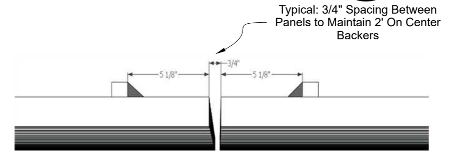
Panel Abutment
