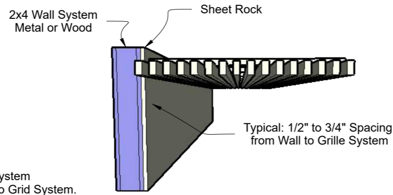
Perimeter View
